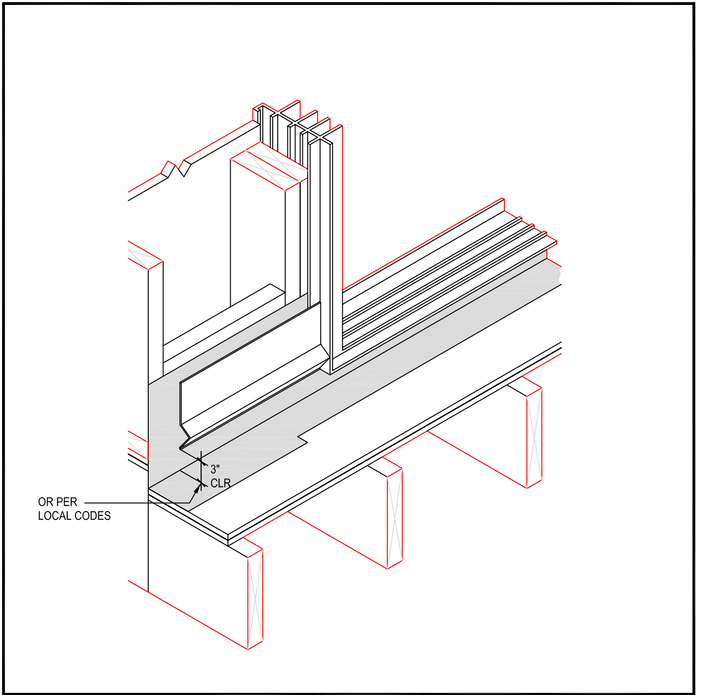
TWO PIECE FLASHING DETAIL
